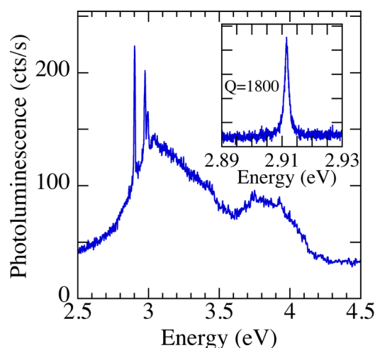
FIG. 2. (Color online) Experimental room temperature spectrum of a modified L3 nanocavity with a lateral shift d = 0.2a . The high-energy recombination feature, around 3.8 eV, is associated with lowest-height QD emission. The low-energy recombination component, around 3 eV, corresponds to large-height QD emission. Inset: spectrum with a high resolution grating (3600 lines/mm) of the lowest-energy mode. A Q factor of 1800 is obtained.
