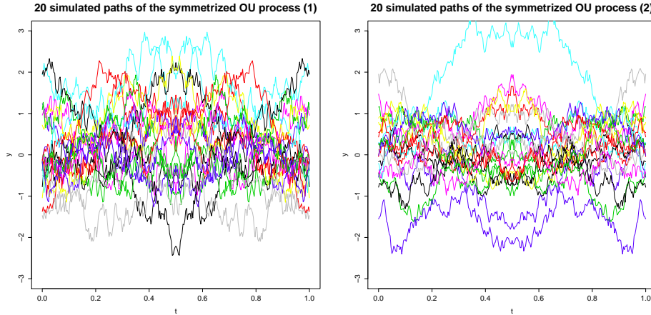
FIGURE 2. Symmetrization of the OU process relying on both kernels defined by eqs. 23, 25. Left: by projection on a fundamental domain (eq. 23). Right: by averaging over the orbits (eq. 25).
