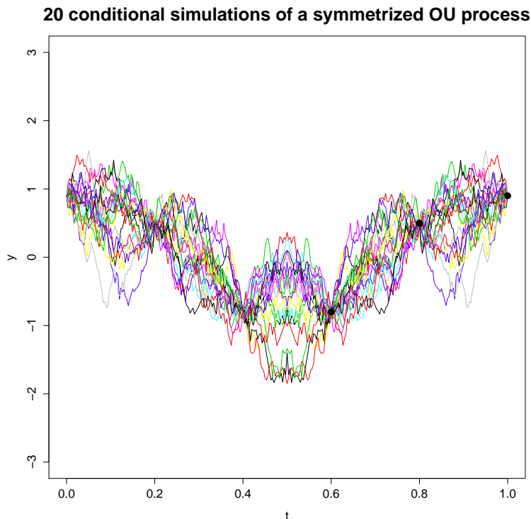
FIGURE 3. Conditional Simulations of the symmetrized OU process with the kernel of eq. 25. The black points stand for the conditioning data.
