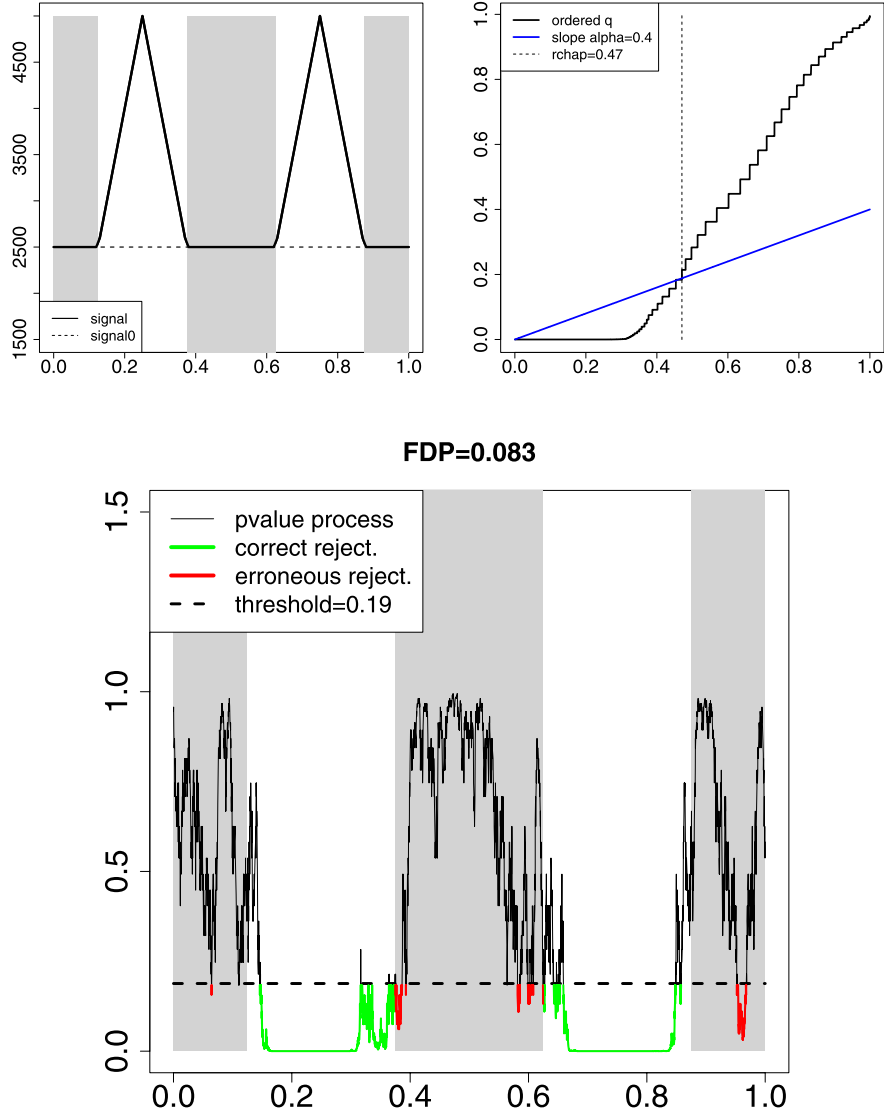
Figure 2. Several plots versus t \in [0, 1] . Top left: \lambda(t) (solid) and \lambda_0 (dashed). Top right: q_{\sigma^{(k)}}(X) and \alpha \sum_{\ell=0}^k w_\ell in function of \sum_{\ell=0}^k w_\ell , for k = 1, \dots, m . Bottom: p -value process p_t(X) defined by (19). \eta = 0.015 , \alpha = 0.4 . The grey areas indicate regions where the null hypotheses are true.
