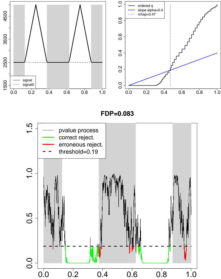
Figure 2. Several plots versus t \in [0,1] . Top left: \lambda(t) (solid) and \lambda_0 (dashed). Top right: q_{\sigma^{(k)}}(X) and \alpha \sum_{l=0}^k w_l in function of \sum_{l=0}^k w_l , for k = 1, \dots, m . Bottom: p -value process p_t(X) defined by (19). \eta = 0.015 , \alpha = 0.4 . The grey areas indicate regions where the null hypotheses are true.
