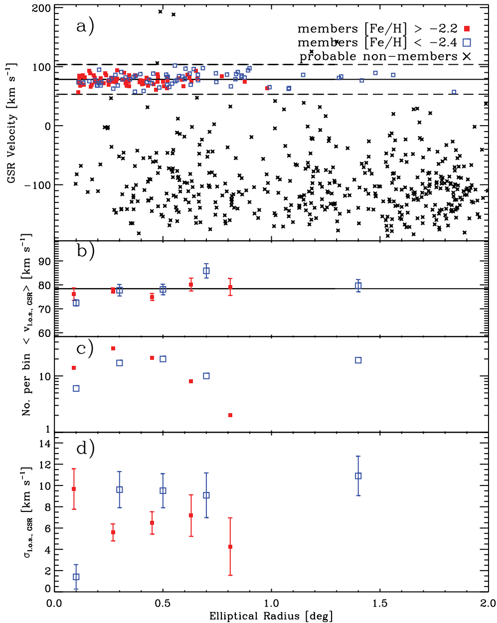
Figure 13. Kinematic properties for probable Sextans members more metal rich than [\text{Fe}/\text{H}] = -2.2 (red filled squares) and more metal poor than [\text{Fe}/\text{H}] = -2.4 (blue open squares). We show the variation of the rotation-subtracted GSR velocity versus elliptical radius (a); average rotation-subtracted GSR velocity (b); number of stars (c); velocity dispersion profile using rotation-subtracted GSR velocities (d). The solid horizontal line indicates the systemic velocity, the horizontal long-dashed lines show the region used for the 3\sigma membership selection.
