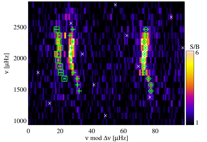
Fig. 9. Échelle diagram of HD 52265, plotted with a folding frequency \Delta\nu = 98.5 μHz. The colour map shows the observed power spectrum normalised by the background (S/B), smoothed over 11 bins. Green symbols with error bars indicate the fitted modes listed in Table 4: plus signs, diamonds, and squares indicate l = 0, 1, and 2 modes, respectively. White crosses indicate orbital harmonics.
