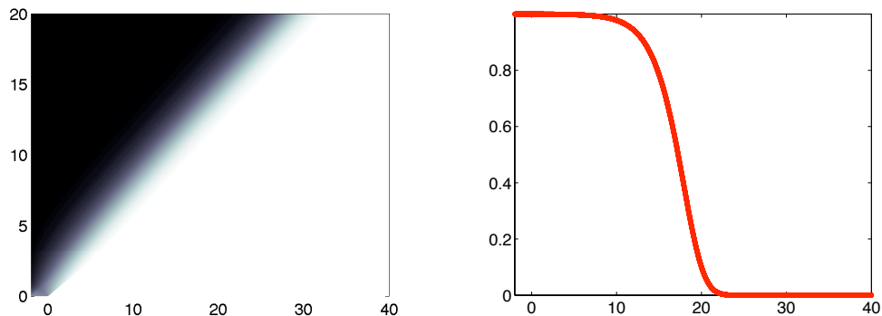
(a) \varepsilon = 1/2
