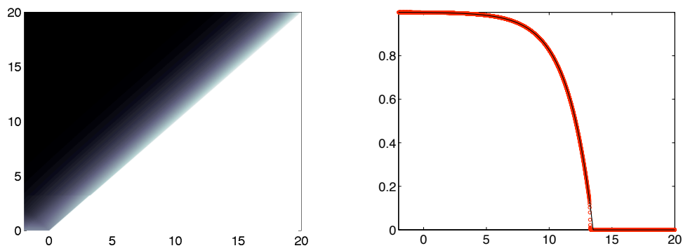
(b) \varepsilon = 1
