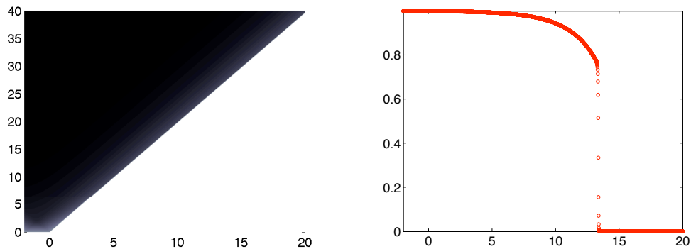
(c) \varepsilon = 2
