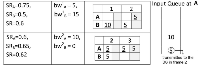
Fig. 3. FIFO Scheduling at SS
