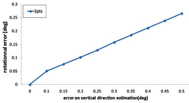
Fig. 10 Impact of the geometric accuracy of the vertical direction on the estimation of (a) the rotation (in degrees), and (b) the base orientation (in degrees) in sideway motion
