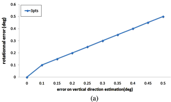
Fig. 11 Impact of the geometric accuracy of the vertical direction on the estimation of (a) the rotation (in degrees), and (b) the base orientation (in degrees) in forward motion
