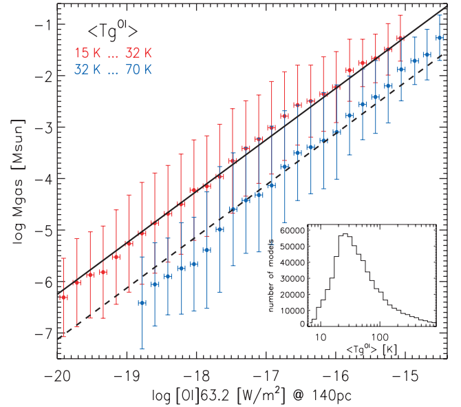
Figure 4. Relation between total disc gas mass and [O I] 63.2 \mu\text{m} line flux at distance 140 pc. The x -axis is subdivided into 30 log-equidistant bins. In each bin, the values of the disc gas mass (parameter, see Table 1) of all models with matching [O I] 63.2 \mu\text{m} line flux are statistically analysed to yield a mean value and a standard variation, which are then plotted as points with vertical error bars. We distinguish between cool and warm models by \langle T_{\text{g}}^{\text{OI}} \rangle as defined in equation (1), and have chosen temperature interval boundaries to bracket the 1\sigma distribution as shown by the inserted histogram. The following models have been selected: dust/gas ratio \rho_{\text{d}}/\rho_{\text{g}} = 0.01 – 1 , flaring index \beta \geq 1 , and inclination angle \leq 60^{\circ} , altogether 122 269 cool and 101 244 warm models. The full and dashed lines show the results from the formula equation (A3) with T_{\text{exc}} = 24 K and T_{\text{exc}} = 30.5 K, respectively.
