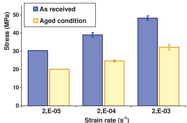
Fig. 8. Influence of the strain rate on the stress obtained when strain = 1%.
