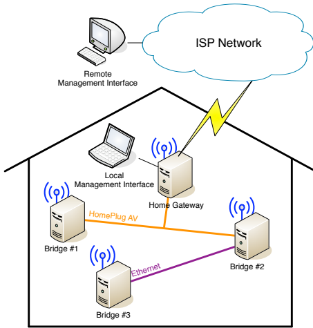
Fig. 6. Supervision architecture
