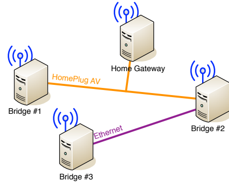
Fig. 7. Testbed network
