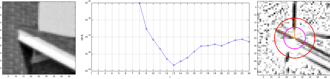
Figure 7: Scale of a junction. Left: image I . The point \mathbf{p} is chosen as the center of I . Middle: for each scale r (in abscissa) is displayed the smallest NFA(j) observed for a junction j of order 3 centered at \mathbf{p} . Right: the smallest scale of detection r_d = 8 in magenta and the scale corresponding to the smallest NFA in red (found for r = 13 ), represented on top of the strength \gamma_{\mathbf{p}}(\mathbf{q}) .
