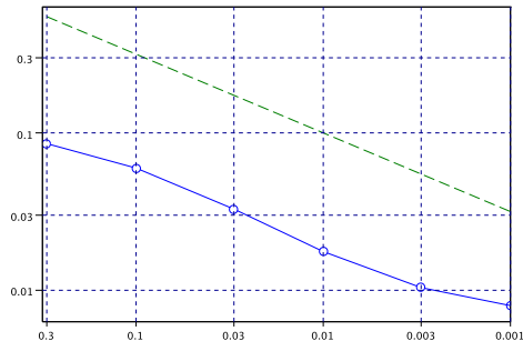
Figure 10: \log \|s_h^\epsilon - s_h\|_{L^1(0,T;L^1(-1,1))} as a function of \epsilon (in blue) and a straight line with slope -1/2 (dashed green). We recover numerically the order of convergence that was expected from (45). Note that the slope of the blue curve is damaged when \epsilon is too large. This phenomenon is due to the fact that the solution is computed on the finite domain x \in (-1, 1) . When the diffusion is large, the boundary conditions affects the numerical solution. The convergence rate is also damaged for small \epsilon . This comes from the fact that the numerical error become comparable to the modeling error \|s^\epsilon - s\| (this effect is particularly visible since the convection is discretized in an implicit way in the scheme presented in Section 3.1 and in an explicit way in the Godunov scheme presented in Section 3.2).
