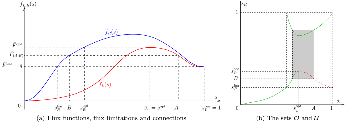
Figure 2: On Figure 2a, the two flux functions f_{L,R} have been plotted. Given a value \bar{F}_{(A,B)} \in [\bar{F}^{bar}, \bar{F}^{opt}] , we construct the unique corresponding connection (A, B) \in \mathcal{U} . On Figure 2b, we have plotted the corresponding sets \mathcal{O} (green solid line) and \mathcal{U} (red dashed line). For a given flux limitation \bar{F}_{(A,B)} , the grey rectangle represents the open set \{(s_L, s_R) \in [0, 1]^2 \mid (f_L(s_L) > \bar{F}_{(A,B)}) \& (f_R(s_R) > \bar{F}_{(A,B)})\} . So, the maximal germ \mathcal{G}_{(A,B)}^* is made of the union of singleton \{(A, B)\} and of the subset \mathcal{O}_{\bar{F}_{(A,B)}} of \mathcal{O} which is outside of the grey rectangle.
