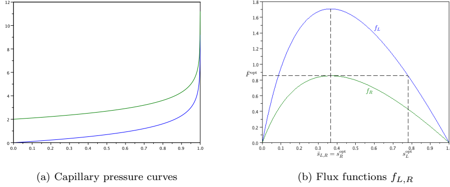
Figure 3: The capillary pressure curves (Fig. 3a) defined by (44)—here P_L = 0 (blue) and P_R = 2 (green)—satisfy \lim_{s \rightarrow 1} \pi_{L,R}(s) = +\infty . Therefore, the maximal extension \tilde{\pi}_{L,R} of \pi_{L,R} is obtained by adding \{0\} \times [-\infty, P_{L,R}) and \{1\} \times \{+\infty\} to the graph \{(s, \pi_{L,R}(s) \mid s \in [0, 1)\} . For the particularly simple choice of parameters and functions done in the simulations, the flux functions f_{L,R} are proportional one to the other. We have represented on Fig. 3b the optimal connection that is relevant for the case presented in Section 3.3.2, but not in the one presented in Section 3.3.3.
