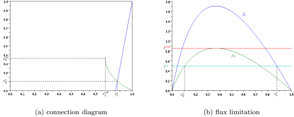
Figure 7: The connection diagram in a case where the intersection of \mathcal{P} (in blue) and \mathcal{U} (in green) is non-empty is presented on Fig. (7a). This results in a flux limitation, in the sense that at the interface, the flux of the hyperbolic solution may not exceed the value \bar{F}^\pi = f_{L,R}(s_{L,R}^\pi) , where (s_L^\pi, s_R^\pi) is the intersection point of \mathcal{U} and \mathcal{P} .
