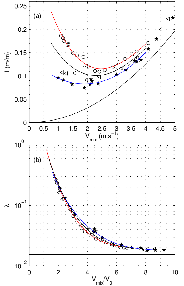
Figure 6: (a): Hydraulic gradient I_h vs. mixture velocity V_{mix} and (b): dimensionless plot of \lambda_h vs. V_{mix}/V_0 , at C = 5\% for \circ : Alumina 6 mm with a fit corresponding to the red line, \star : Glass 5 mm with a fit corresponding to the blue line and \triangleleft : mixture 3. The black solid line is the mean of the two fits.
