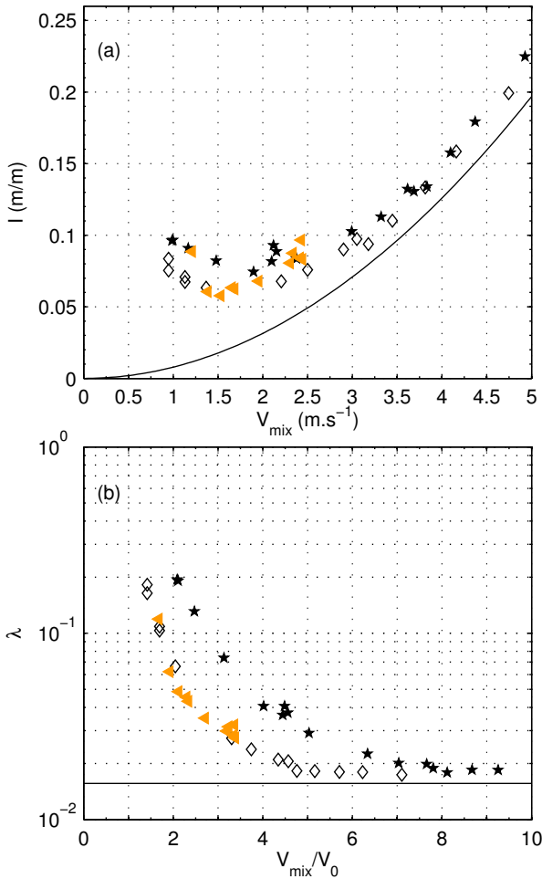
Figure 8: (a): Hydraulic gradient I_h vs. mixture velocity V_{mix} and (b): dimensionless plot of \lambda_h vs. V_{mix}/V_0 , at C = 5\% for \star : Glass 5 mm, \diamond : Glass 10 mm and orange \triangleleft : stones.
