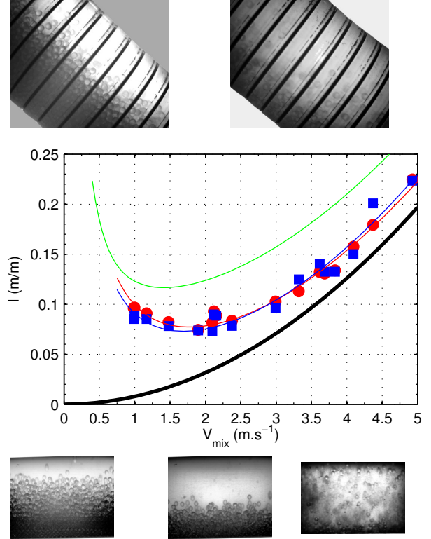
Figure 3: Illustration of the different regimes. Hydraulic gradient vs. V_{mix} . Glass beads of 5 mm, C = 5\% . Solid black line: water flowing alone I_f , red \bullet : I_h , blue \blacksquare : I_s . The blue and red solid lines are fits of the type a/V_{mix} + bV_{mix}^2 (see § 3.3). The green solid line stands for I_v predicted with the model developed for vertical pipelines (see § 3.1).
