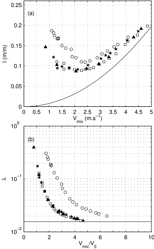
Figure 5: (a): Hydraulic gradient I_h vs. mixture velocity V_{mix} and (b): dimensionless plot of \lambda_h vs. V_{mix}/V_0 , at C = 5\% vs. for \circ : Alumina 6 mm, \square : Alumina 15 mm, \triangle : mixture 1 and \star : mixture 2.
