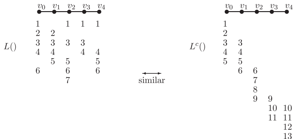
Fig. 1. Example of a list L which is similar to a waterfall list L^c .
