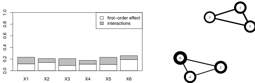
Figure 1: Sensitivity analysis of the example experiment. First-order and total Sobol indices (left), total interaction indices (right).
