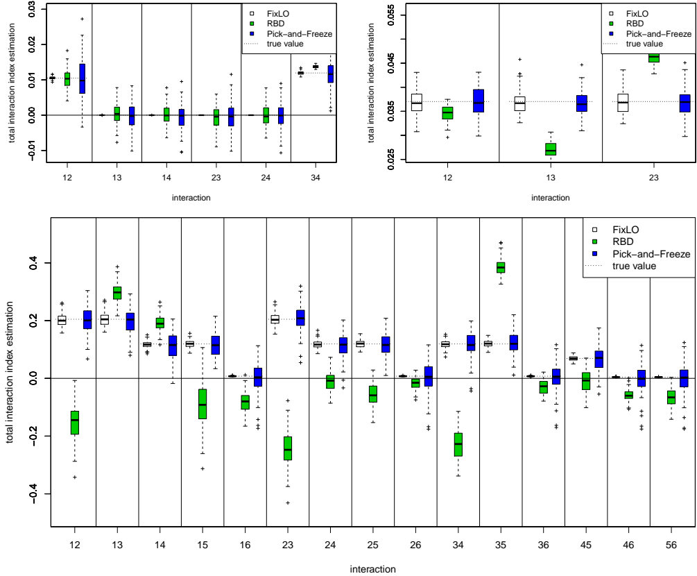
Figure 2: Estimates of the TII by the three estimators (20), (22), and (23) for test functions 1 (top left), 2 (top right) and g -function (bottom).
