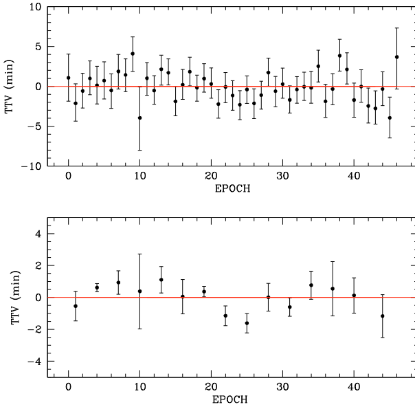
Fig. 6. Top: median value and 1- \sigma limits of the TTV posterior distributions obtained in MCMC3 . Bottom: same curve obtained after binning the TTVs per three (error of each bin = error on the mean).
