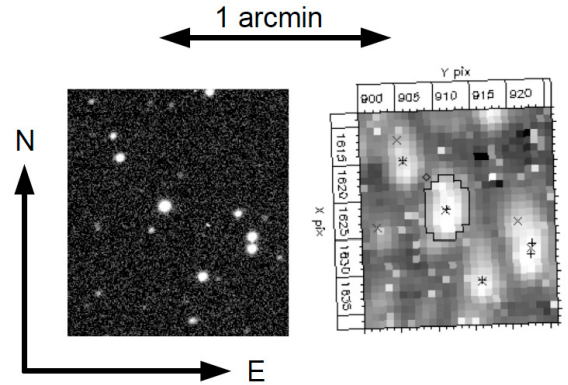
Fig. 2. The sky area around CoRoT-12 (brightest star near the centre). Left: R -filter image with a resolution of 1.3'' taken with the INT/WFC. Right: image taken by CoRoT, at the same scale and orientation. The jagged outline in its center is the photometric aperture mask; indicated are also CoRoT's x and y image coordinates and positions of nearby stars from the Exo-Dat (Deleuil et al. 2009) database.
