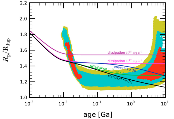
Fig. 8. Evolution of the size of CoRoT-12b (in Jupiter units, R_{\text{Jup}} ) as a function of age (in billion years), compared to constraints inferred from CoRoT photometry, spectroscopy, radial velocimetry and CESAM stellar evolution models. Red, blue and yellow-green dots correspond to the planetary radii and ages that result from stellar evolution models matching the inferred \rho_* - T_{\text{eff}} uncertainty ellipse within 1\sigma , 2\sigma and 3\sigma , respectively. Planetary evolution models for a planet with a solar-composition envelope and no core are shown as plain lines and are labeled as follow: standard (black): irradiated planet with no extra heat source; opacities \times 30 (blue): opacities have been artificially multiplied by 30 compared to standard model; dissipation : models in which 10^{26} (green), 10^{27} (pink), and 10^{28} (purple) \text{erg s}^{-1} is deposited at the planet’s center. These models assume a total mass of 0.92 M_{\text{Jup}} and an equilibrium temperature of 1450 K
