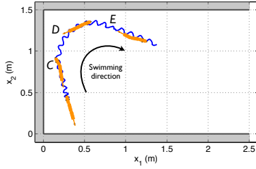
Fig. 10. The preset robot trajectory for the turning within a corner test. The blue line is the trajectory of the head module.
