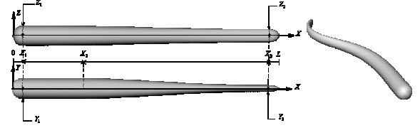
Figure 3: Geometric shape of the eel-like prototype,
