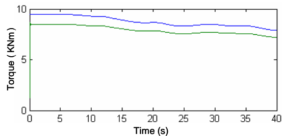
Fig. 10. Torque: Reference (blue) and real (green).
