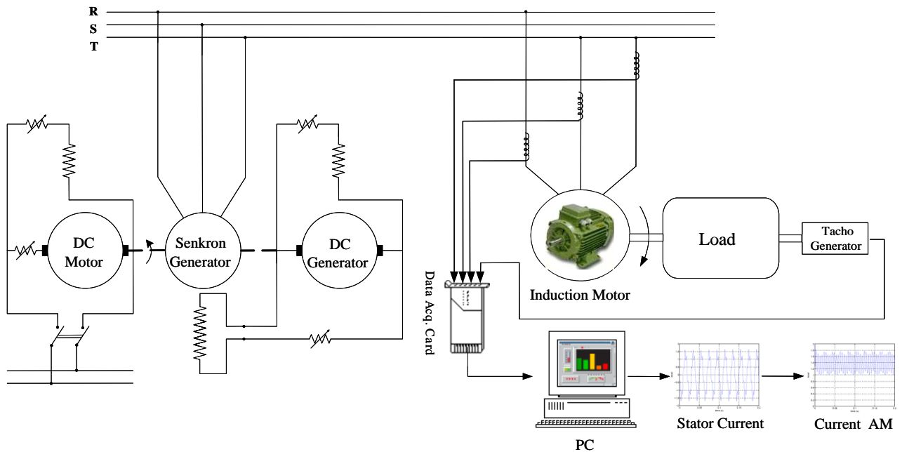
Fig. 6. Test facility.
