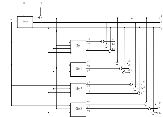
Fig. 4. GOS Structure
