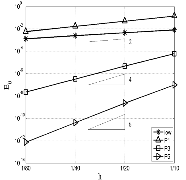
Figure 1: Example 1 — convergence curves of E_0 for the exponential function using a uniform mesh with Pe=1 .
