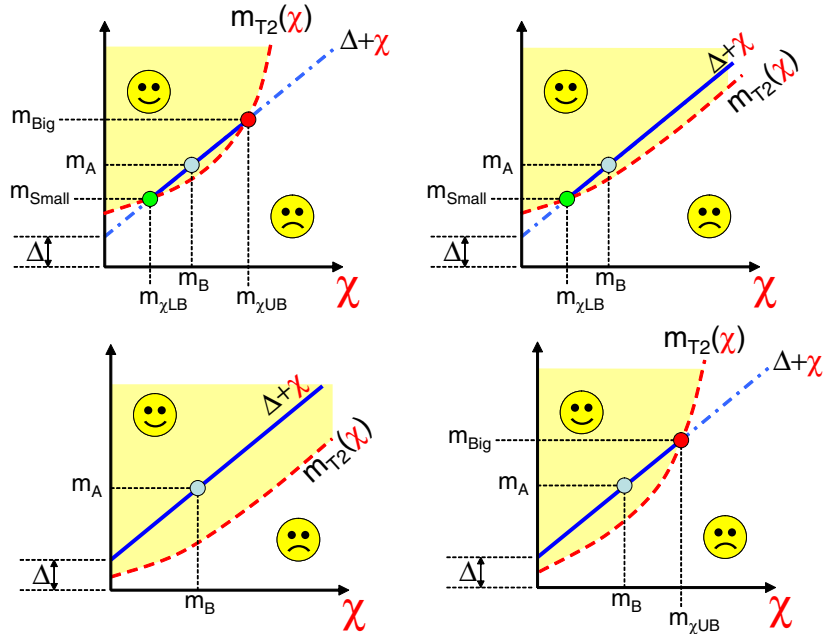
FIG. 19: The four potential combinations of constraint coming from M_{T2} and the dilepton edge which together contribute to M_{2C} are shown. The mass difference \Delta = m_A - m_B is assumed to have been measured independently, e.g. from the endpoint of the dilepton invariant mass distribution in three-body decays A \rightarrow B\ell^+\ell^- . Knowledge of \Delta constrains the (m_A, m_B) solution to lie on the diagonal line. The constraint from the pair decay kinematics gives the separate M_{T2} constraint, for which the solution must lie above and to the left of the dashed line. The intersection of the shaded region with the diagonal line then gives an event-by-event allowed solution space.
