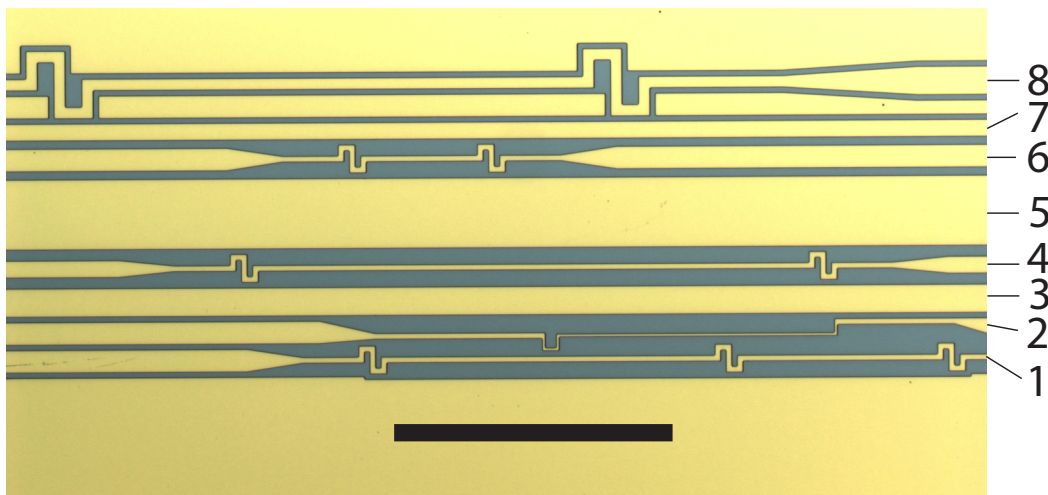
Figure 1. (Colour online) Optical microscope image of the central section of an atom chip. The chip hosts a series of micro-wires of various geometries for creating one-dimensional traps and box-shaped potentials. The length of the scale bar is 500 \mu\text{m} . The numbers at the right identify the atom chip wires and correspond to the numbers in Table 1.
