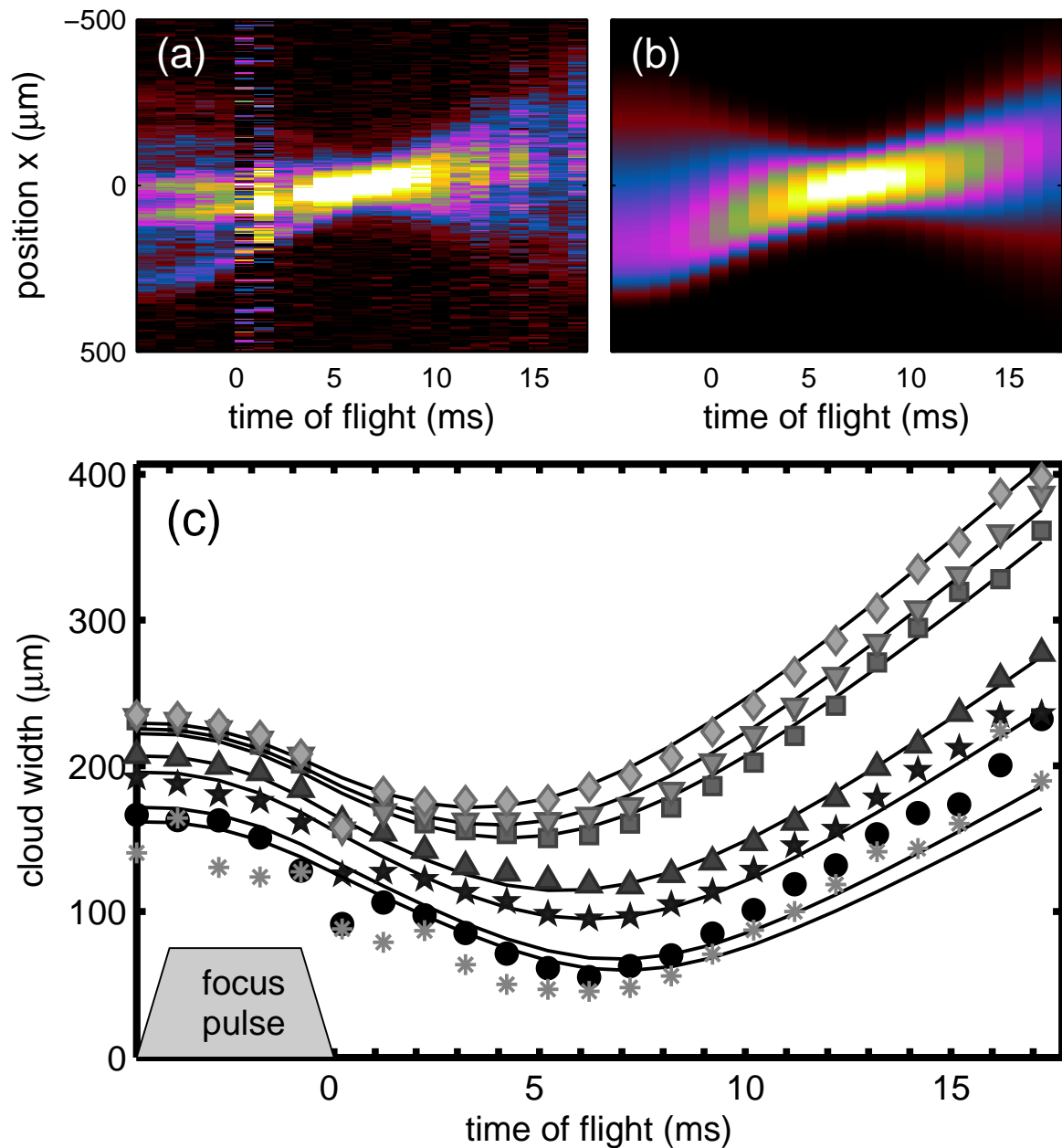
Figure 5. (Colour online) Focusing ultracold atoms from a box-shaped potential. (a) Measured optical density profiles during the focus sequence. (b) Calculated profiles based on the focusing model of Eq. (7). (c) Cloud width during the focus sequence for several values of the final evaporation radio frequency and corresponding fits used to determine the cloud temperature. Symbols (curves) correspond to final radio frequencies (fitted temperatures) of \diamond 1.80 MHz (4.16 \mu\text{K} ), \nabla 1.70 MHz (3.44 \mu\text{K} ), \square 1.64 MHz (2.95 \mu\text{K} ), \triangle 1.50 MHz (1.51 \mu\text{K} ), \star 1.46 MHz (1.02 \mu\text{K} ), \bullet 1.42 MHz (0.42 \mu\text{K} ) and * 1.41 MHz (0.28 \mu\text{K} ). The shape and duration of the focus pulse is indicated by the shaded area.
