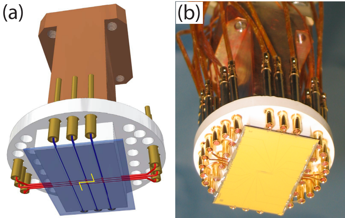
Figure 3. (Colour online) (a) Chip mount showing the arrangement of the two layers of miniwires. The orientation of the Z-wire is indicated at the center of the drawing. (b) Photograph of the completed atom chip construction.
