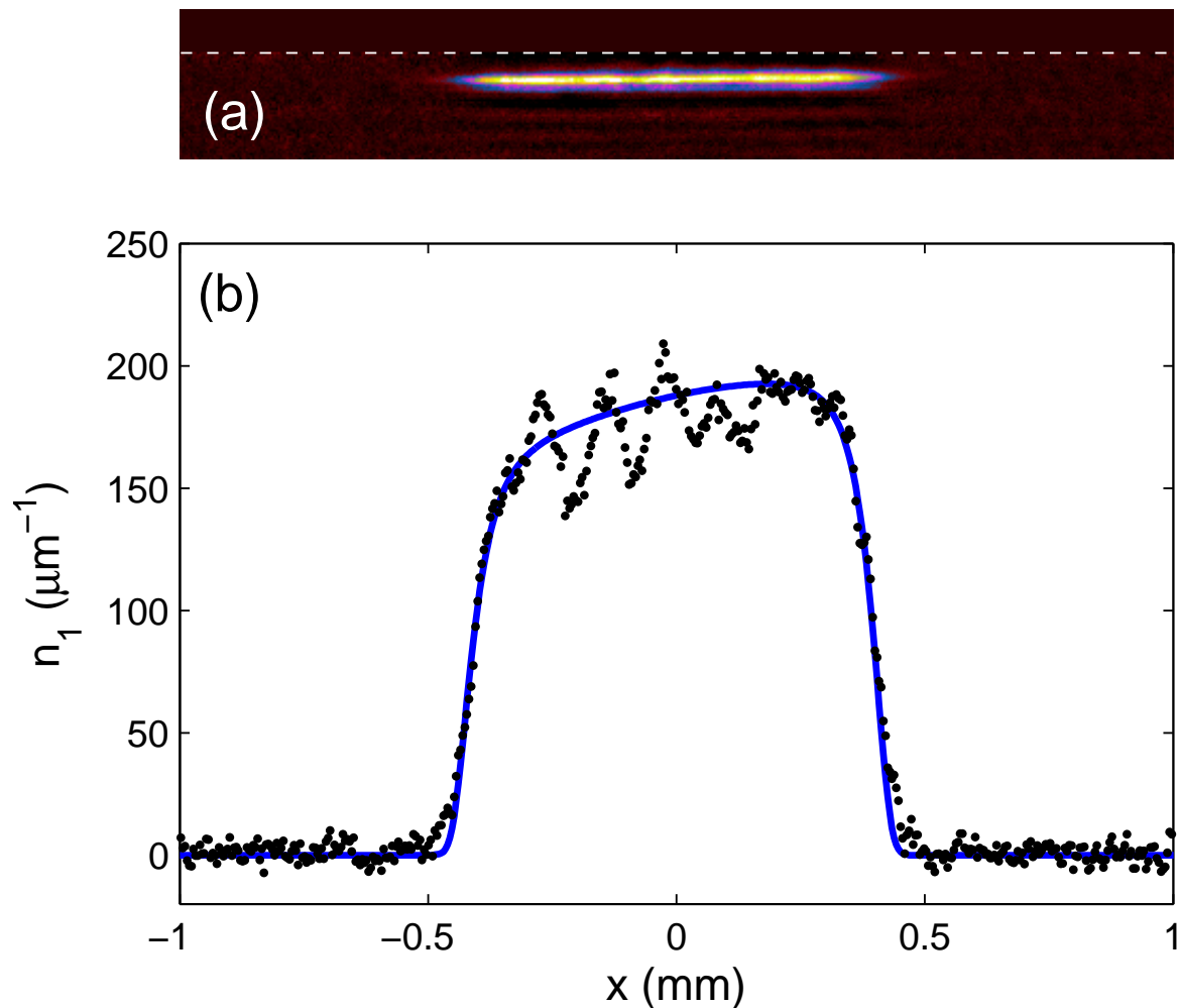
Figure 4. (Colour online) In-situ atomic density distribution after loading the box-shaped potential for a final evaporation radio frequency of 1.80 MHz. (a) Optical density image showing a 70 \times 465 pixel region ( 4.3 \mu\text{m} pixel size in the object plane). The dashed line indicates the approximate position of the chip surface. (b) Integrated profile showing the corresponding linear atomic density n_1 as a function of longitudinal position x . The solid line is a result from the analysis of Sec. IVc for the expected in-trap density distribution corresponding to a temperature of T = 4.16 \mu\text{K} .
