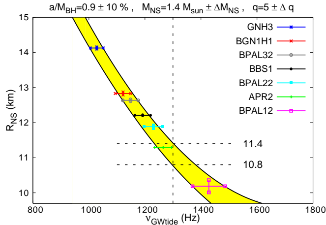
Figure 4. R_{NS} versus \nu_{GWtide} is plotted for M_{NS} = 1.4M_{\odot} \pm \Delta M_{NS} , q = 5 \pm \Delta q and a/M_{BH} = 0.9 \pm 10\% . The black continuous lines are the parabolic fits of the extreme points of the horizontal error bar for each EOS. The vertical dashed line corresponds to a supposed detected value of \nu_{GWtide} equal to 1300 Hz; the two horizontal dashed lines identify the uncertainty on the evaluation of R_{NS} .
