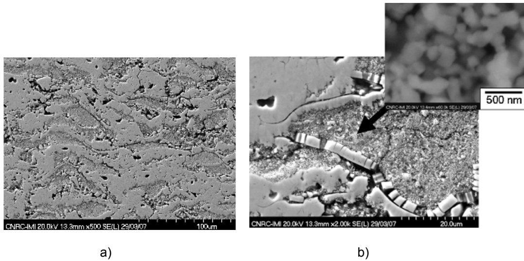
Figure 18. a) Plasma-sprayed coating (cross-section) engineered from the nanostructured agglomerated YSZ particles (Figs. 13 and 17) by employing the in-flight particle characteristics described in Fig. 16. b) High magnification view showing a semi-molten nanostructured agglomerate (porous nanozones) embedded in the coating microstructure [130].
