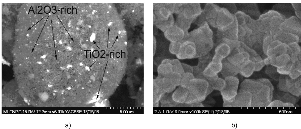
Figure 14. a) Spray-dried agglomerated Al 2 O 3 -13wt%TiO 2 particle. b) Higher magnification view showing the "ultra-fine" character of the agglomerate [89].
