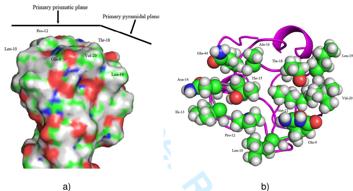
Figure 1. a) Surface view of the compound ice-binding surface (IBS) of type-III AFP. The primary prismatic and pyramidal plane binding sections of AFP are indicated, along with some of the residues identified at the IBS (Gln-9, Leu-10, Pro-12, Thr-18, Leu-19 and Val-20). b) Ribbon representation of type-III AFP with all the compound ice-binding surface residues given as space-filled spheres (Gln-9, Leu-10, Pro-12, Ile-13, Asn-14, Thr-15, Ala-16, Thr-18, Leu-19, Val-20, Met-21, Gln-44). Residues are colored as follows: nitrogen = blue, oxygen = red, carbon = green, and deuterium = grey.
