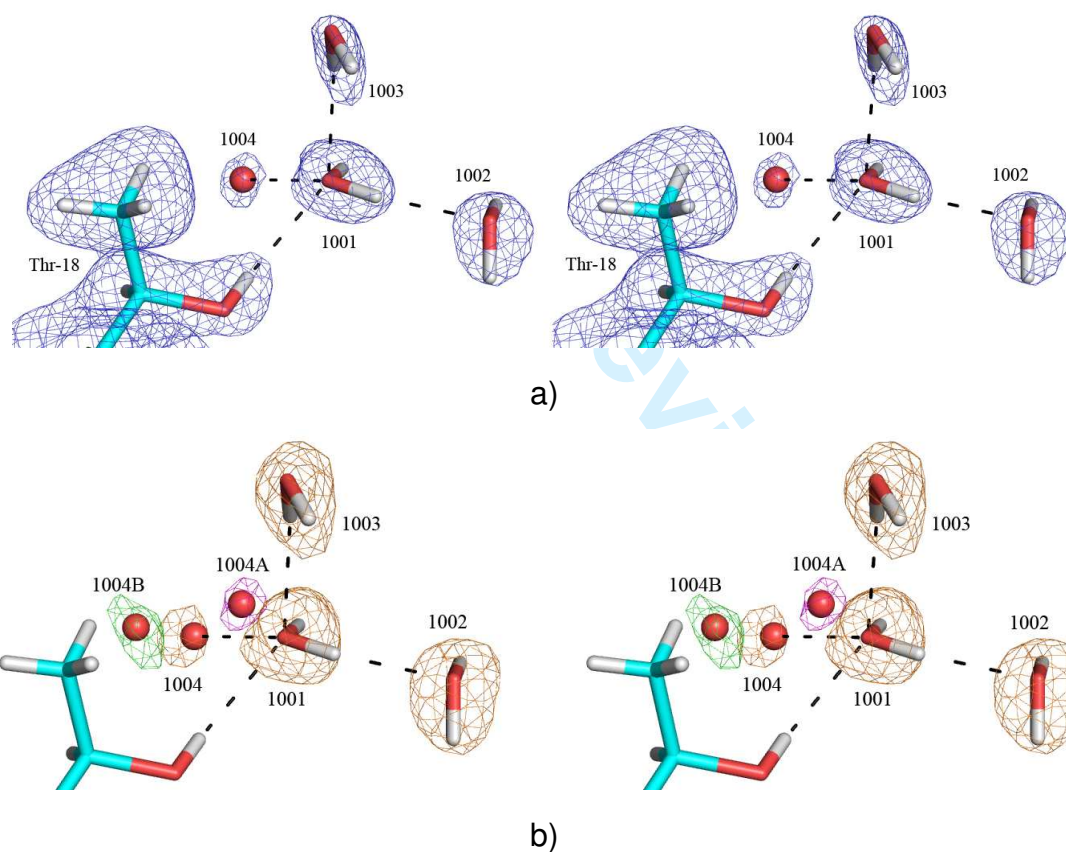
Figure 5. Superposition of the tetrahedral water cluster model and density maps.
