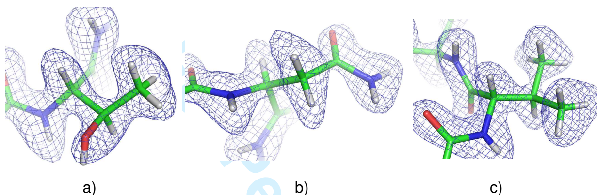
Figure 2. \sigma_A -weighted 2F_o - F_c nuclear scattering density maps (contour level = 1.6 r.m.s.) for AFP D at 1.85Å resolution. a) Threonine-53. b) Asparagine-8. c) Valine-5. The orientations of the side-chains of amino-acid residues (e.g. methyl- and hydroxyl groups) are clearly seen due to the high quality of the nuclear scattering density maps obtained when using perdeuterated samples for data collection.
