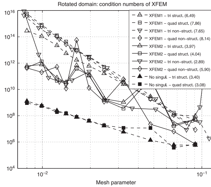
Figure 22. Second test-case , condition numbers of all XFEM (with/without singular enrichment).
