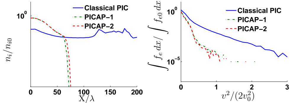
Figure 21: Plasma expansion test case. Simulation 4: space and time under-resolved case: \Delta x = 4\lambda and \Delta t = 3\omega_i^{-1} and small number of particles (1000 particles per mesh and per species). Ion density as a function of position in log scale (left) and electron velocity distribution as a function of v^2/(2v_0^2) (right) with Classical PIC and PICAP schemes, at time t = 30\omega_i^{-1} .
