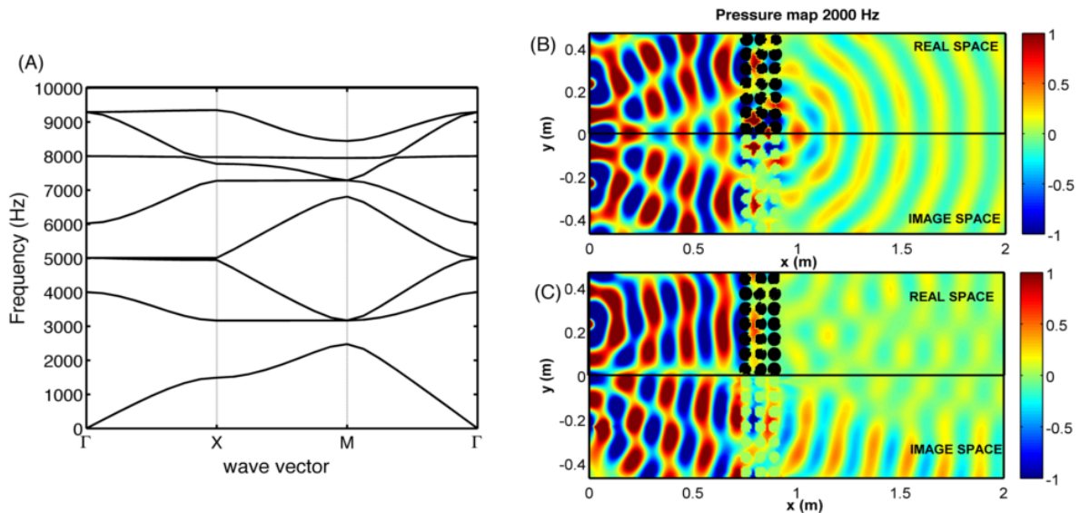
Figure 4. (Colour online) Pressure maps for an array of 7 \times 3 scatterers in square array with lattice constant a = 0.069 m considering a line source placed at point O = (0, 0.235) m. The circular scatterers present a radius r = 0.0275 m. For these simulations we have considered H_y = 0.755 m and H_x = 0.0275 m. (A) Band structure calculated using the PWE method. (B) and (C) pressure maps ( Re(P) ) (Pa) at 2000 Hz for an acoustically-hard ground and an finite impedance ground ( \sigma_e = 4000 Pa s/m 2 and \alpha_e = 105 m -1 ) respectively.
