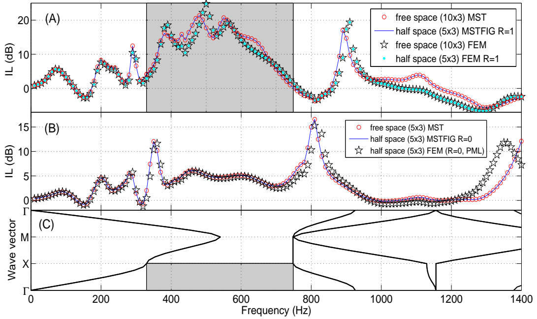
Figure 2. (Colour online) Predicted IL spectra of a square array of rigid cylinders with diameter 0.25 m, lattice constant 0.3 m above ground plane at y = 0 and 'lowest' cylinder centres at H_x = 0.15 m. The source and receiver coordinates are (0,0) m and (2.5,0) m respectively. The nearest part of the array is at H_y = 1 m from the source. (A) Acoustically-hard ground R(\vec{r}_O, \vec{r}_R, \nu) = 1 : Blue continuous line (respectively, green dots) shows the IL produced by a 5 \times 3 square array of rigid cylinders calculated using the MSTFIG (respectively, finite element method). The open red circles (respectively, black pentagrams) show the IL produced by a doubled (i.e. a 10 \times 3 ) lattice in the free field calculated using the MST (respectively, finite element method). (B) Completely absorbent ground R(\vec{r}_O, \vec{r}_R, \nu) = 0 : Blue continuous line (respectively, open red circles and black pentagrams) shows the IL produced by a 5 \times 3 square array of rigid cylinders calculated using the MSTFIG (respectively, MST and FEM). (C) Band structure in the considered case calculated using plane wave expansion (PWE). The grey area represents the pseudogap in \Gamma X direction.
