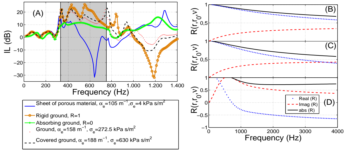
Figure 3. (Colour online) IL and reflection coefficient predictions obtained using the MSTFIG for five values of ground impedance. (A) IL of the same array as in Figure 2A with the source and the receiver placed at points (0,0.25) m and (2.5, 0.75) m respectively, and H_x = 0.15 m and H_y = 1 m. The orange continuous dotted line shows the IL predicted in the case of a rigid ground. The green crossed dash line shows the IL predicted in the case of a completely absorbent ground. The black dashed line shows the IL predictions in the case of a covered ground characterized by \sigma_e = 630 kPa s/m 2 and \alpha_e = 188 m -1 . Red dots show the IL predicted for the case of a ground characterized by \sigma_e = 272500 Pa s/m 2 and \alpha_e = 158 m -1 . The blue continuous line shows the IL predictions in the case of a sheet of porous material characterized by \sigma_e = 4000 Pa s/m 2 and \alpha_e = 105 m -1 . The real, imaginary and absolute values of the reflection coefficients of these three grounds are shown in (B), (C) and (D) respectively. The grey area represents the pseudogap in \Gamma X direction.
