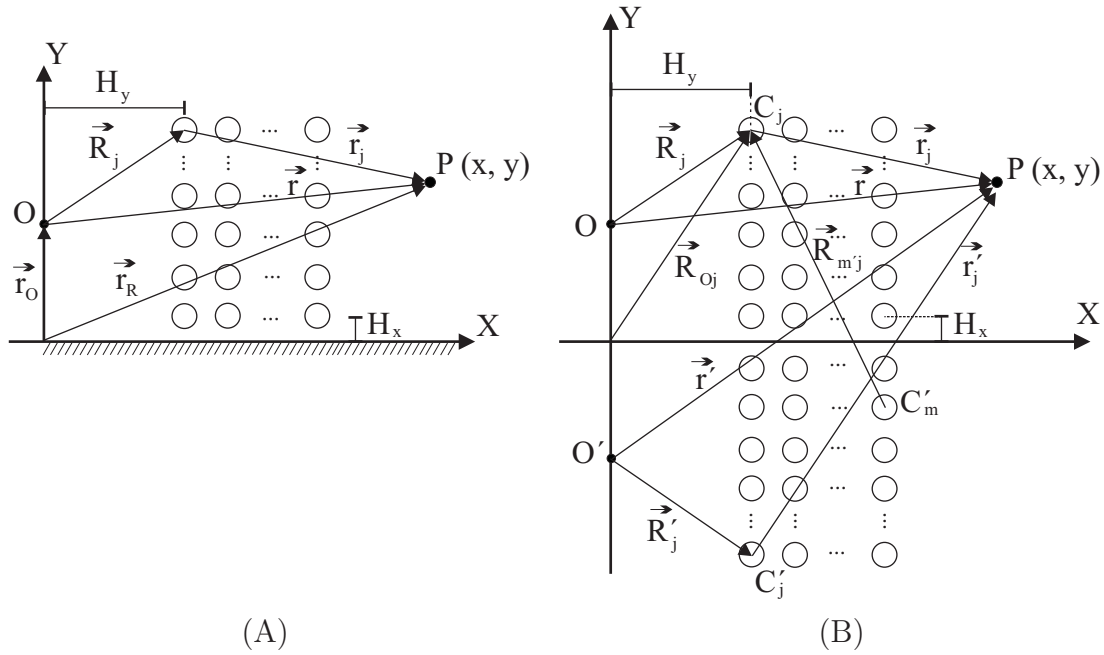
Figure 1. (A) Square lattice array above a perfectly reflecting plane. (B) Schematic of the real and the image sources and the real and the image scatterers.
