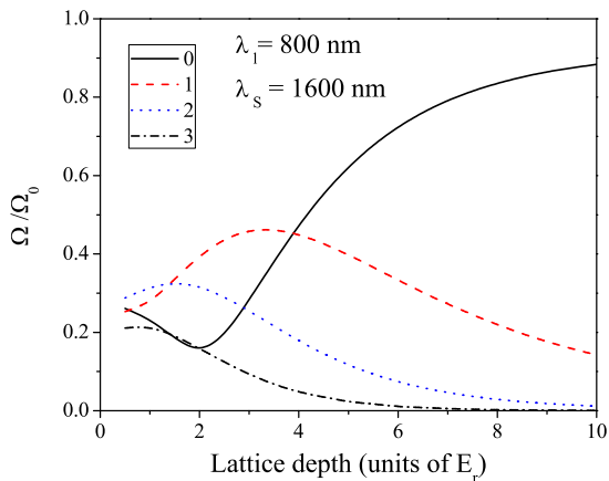
FIG. 4: Coupling strengths \Delta m = 0, \pm 1, \pm 2, \pm 3 versus lattice depth for a lattice wavelength \lambda_l = 800 nm and tilted Raman beams giving an effective wavelength of \lambda_s = 1600 nm.
