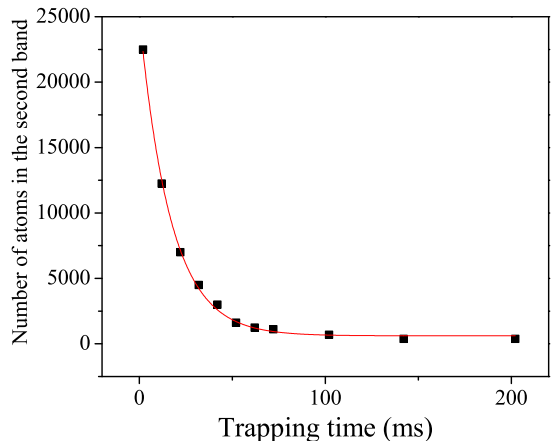
FIG. 12: Population in the first excited band as a function of trapping time. The solid line is an exponential decay fit to the data from which we extract a lifetime of 16 ms.
