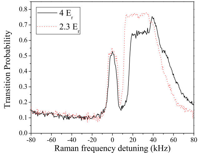
FIG. 11: Transition probability as a function of Raman frequency. The broad peak at vanishing relative Raman laser detuning ( \nu_{R\text{veg}} = 0 corresponds to unresolved intersite transitions in the same lattice band. The large structure arising between 10 and 50 kHz is due to a coupling from the bottom to the first excited band.
