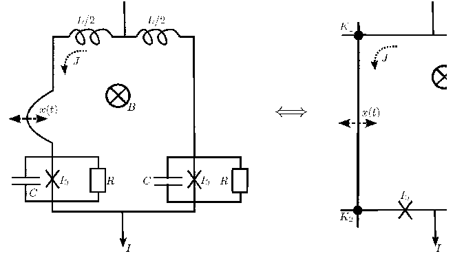
Fig. 1: The scheme of a nanomechanical oscillator embedded into a SQUID circuit. The assumption of this work is to consider the scheme a) as being equivalent to the scheme b) (for representation simplicity, we drop the self-inductance L , capacitance C and resistance R on the b) subfigure). In particular, this assumption allows us to disregard the elastic properties of the bar, and to use relativistic arguments when the bar and circuit are two different sub-systems of the entire circuit.
