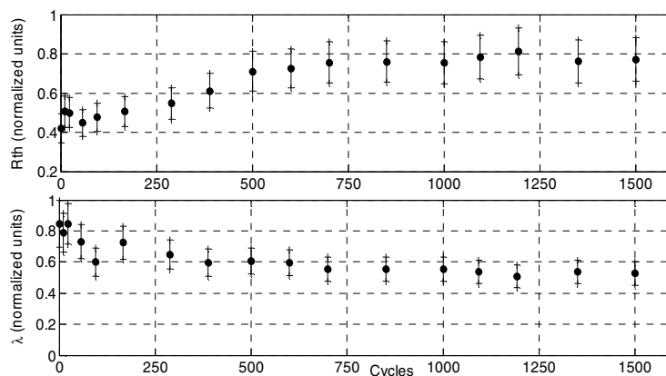
Figure 11: Evolution of the Hiflow 300P thermal resistance and conductivity versus cycles number.
