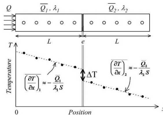
Figure 6: Thermal characterization principle.
