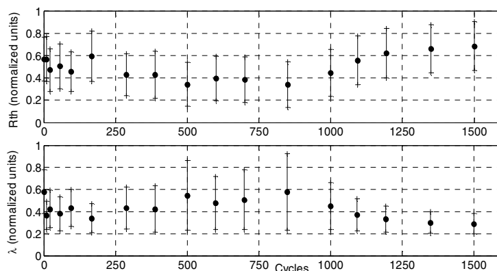
Figure 9: Evolution of the Compelma T014 thermal resistance and conductivity versus cycles number.
