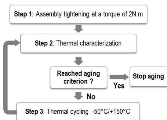
Figure 3: Schematic aging protocol.
