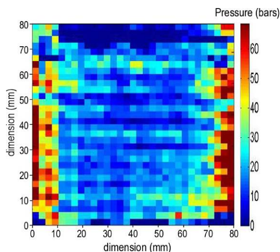
Figure 2: Pressure distribution.
