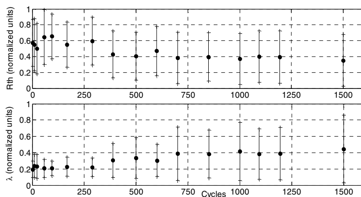
Figure 10: Evolution of the Egraf 1205A thermal resistance and conductivity versus cycles number.
