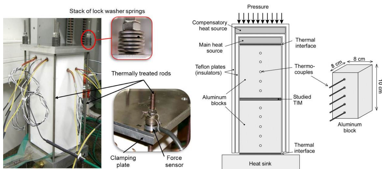
Figure 1: Experimental set-up.
