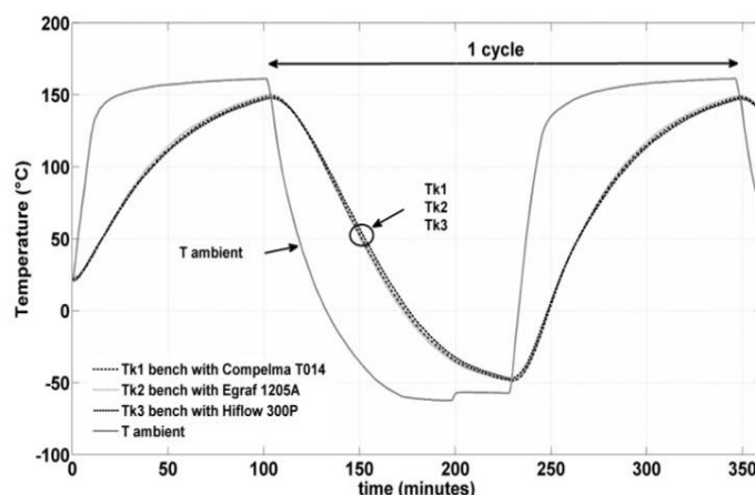
Figure 5: Temperature profile on a cycle.
