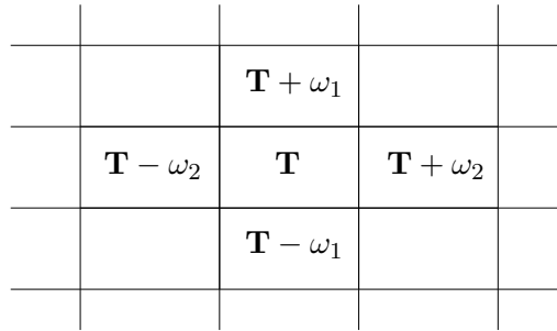
FIGURE 6. Informal construction of the universal covering
