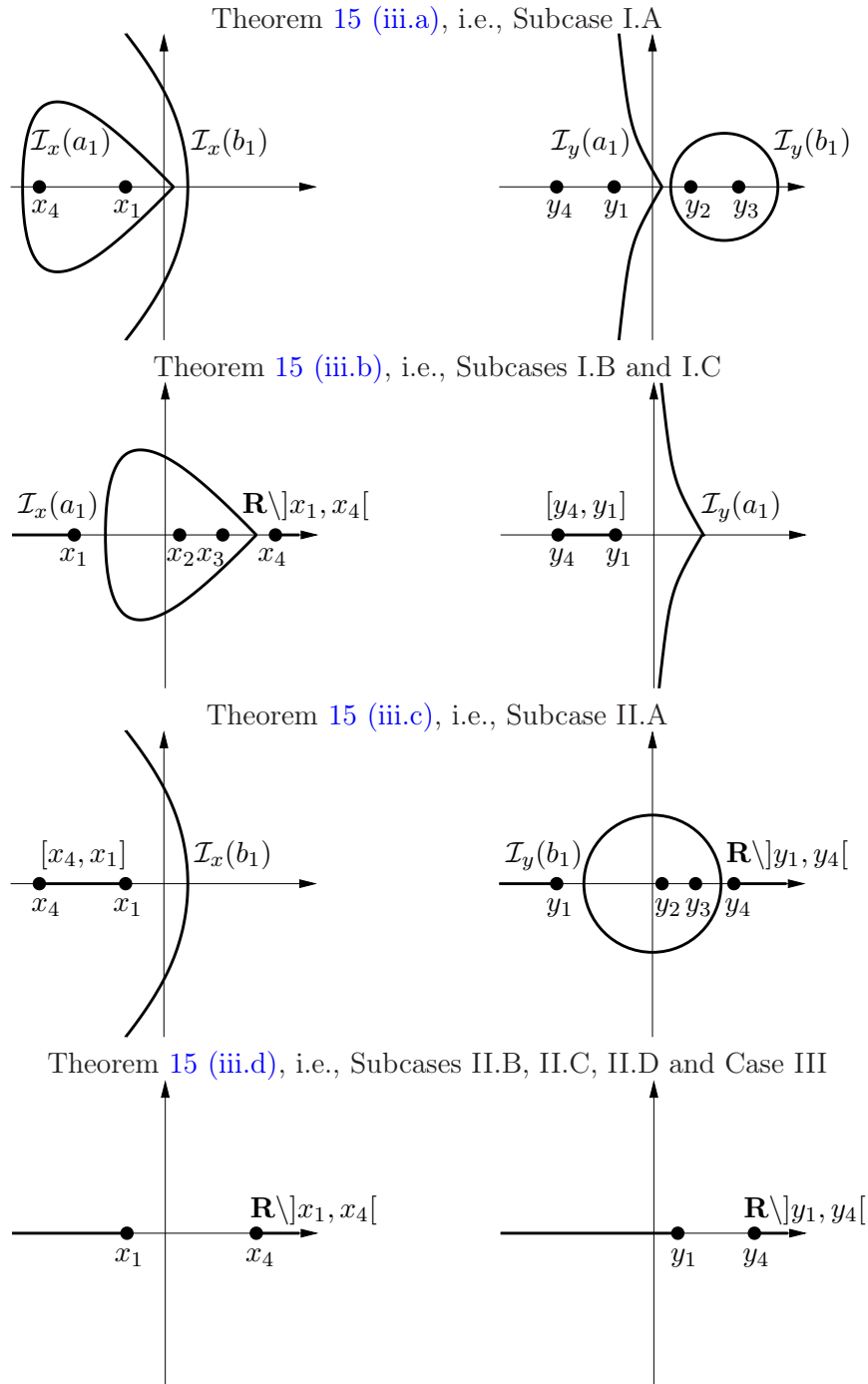
FIGURE 11. For walks pictured on Figure 17, curves where poles of the set of branches of x \mapsto Q(x, 0) and y \mapsto Q(0, y) are dense
