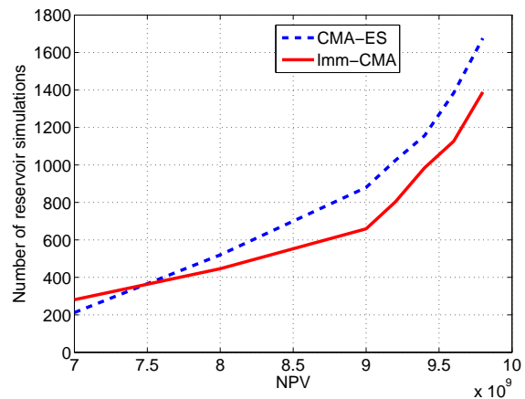
Fig. 9 The mean number of reservoir simulations needed to reach a given NPV value using CMA-ES with meta-models ( solid line ) and CMA-ES ( dashed line ). Ten runs are performed for each algorithm.
