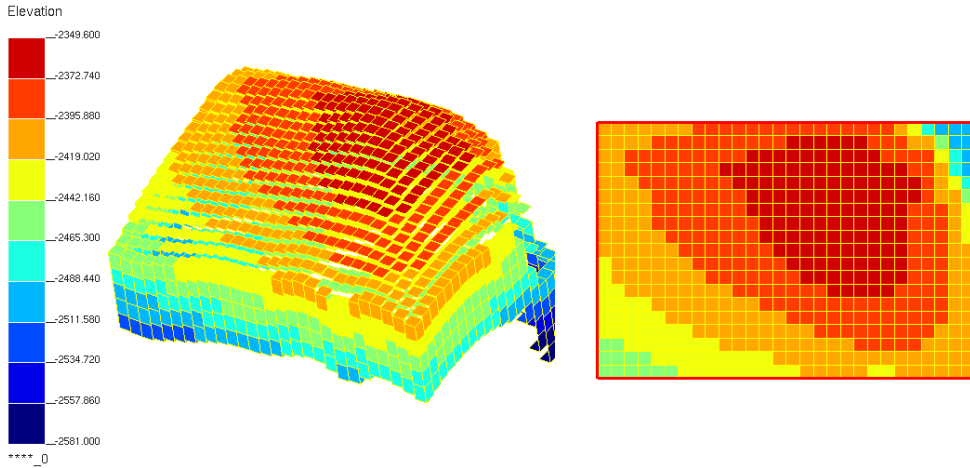
Fig. 3 Elevation (in meters) and geometry of the PUNQ-S3 test case.
