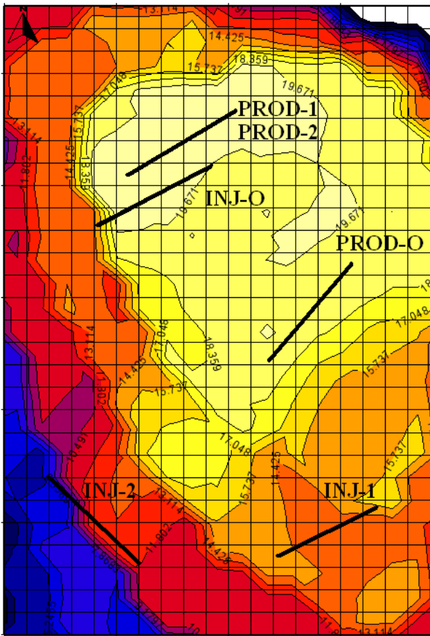
Fig. 10 The SoPhiH Map, with solution well configuration obtained using CMA-ES with meta-models (PROD-O, INJ-O) and two engineer’s proposed well configurations (PROD-1, INJ-1 and PROD-2, INJ-2).
