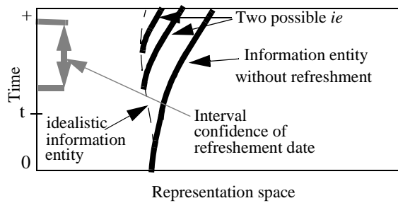
Fig. 15. Illustration of refreshment modeling based on a time confidence interval.
