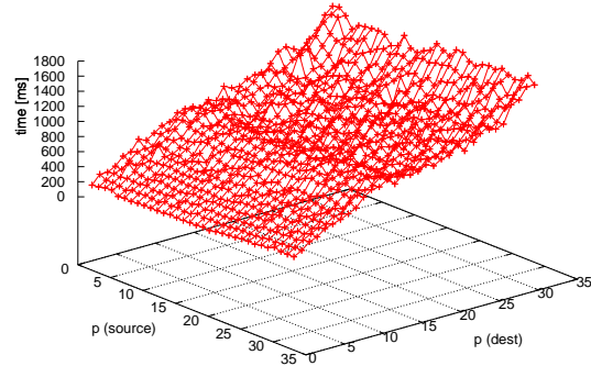
Figure 4. Data redistribution overhead. p(src) : number of source processors. p(dst) : number of destination processors.
