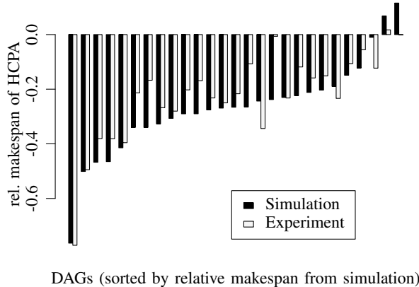
Figure 7. HCPA makespan relative to that of MPCA using empirical models. Left-hand side: n = 2,000 . Right-hand side: n = 3,000 .
