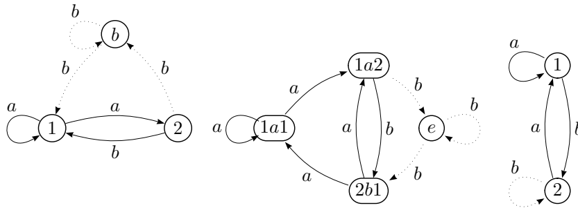
Figure 13: Another embedding of the previous automaton.
