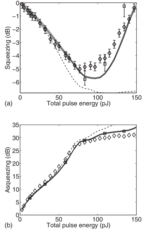
FIG. 11. Squeezing degradation at high intensity: (a) squeezing and (b) antisqueezing measurements for L=13.35 m of fiber I. Solid and dashed lines show the simulation results with and without Raman effects (i.e., a purely electronic nonlinearity), respectively. The data points marked by squares are the results of exact +P calculations with error bars indicating estimated sampling error. The points at 109 and 134 pJ were calculated with 10 000 trajectories; the other 4 +P points were calculated with 1000 trajectories. Note that these results were obtained in an experimental setup with higher losses than that of Fig. 7, giving a reduced magnitude of raw squeezing. The simulations here assume 19.9% loss.
