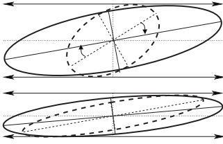
FIG. 8. Illustration of the effect of excess phase noise on different squeezing ellipses. Dashed line gives the Kerr-squeezed ellipse and the solid line gives the ellipse with added phase noise. The effect on the squeezing and the angle is less for the ellipse with larger Kerr squeezing (lower ellipse).
