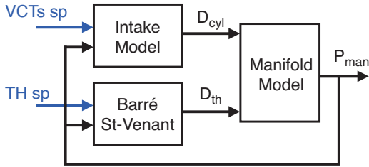
Figure 22 Pressure prediction scheme.
