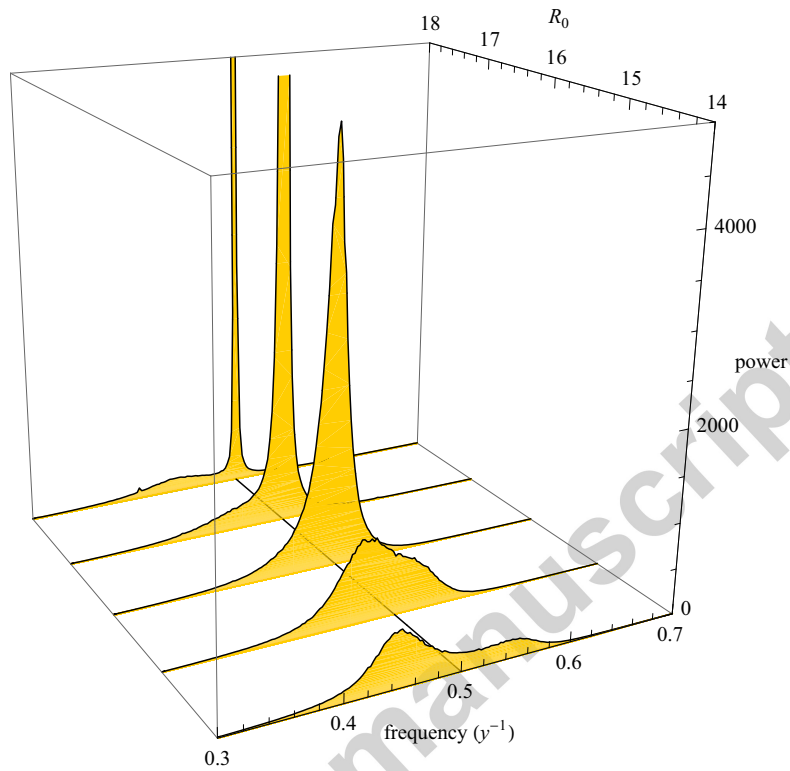
Figure 8: Simulation results showing how the power spectrum of the stochastic oscillations changes as the period doubling bifurcation point is crossed. The peaks for R_0 = 17 and 18 have been cropped for clarity.
