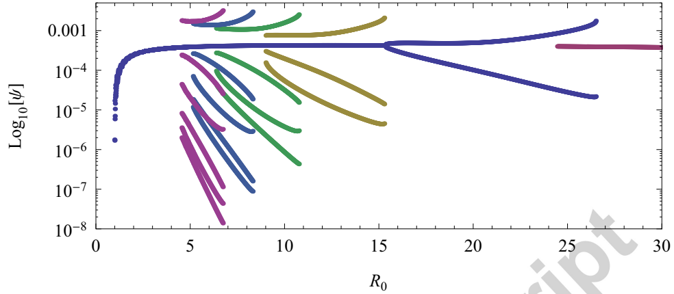
Figure 4: Bifurcation diagram showing the SIR dynamics as a function of R_0 . Fixed parameters: \beta_1 = 0.29 , \gamma = 1/13 , \mu = 5.5 \times 10^{-5} and \eta = 0 . The different period limit cycles are shown in different colours, which are produced by different initial conditions.
