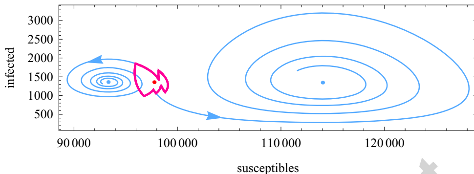
Figure 1: Phase portrait illustrating a deterministic solution of the forced SIR model. The term-time forcing creates a limit cycle (red curve) as the system alternately spirals between the two fixed points defined by \beta_H = \beta_0(1 + \beta_1) and \beta_L = \beta_0(1 - \beta_1) . The light blue solutions show the behaviour if the forcing was switched off, to illustrate the two spiral attractors. The red dot shows the fixed point calculated using the approximation where \beta(t) is replaced by \langle \beta \rangle .
