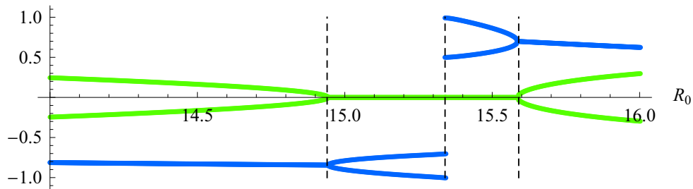
Figure 6: Floquet multipliers near to the period doubling bifurcation point, showing the virtual-Hopf pattern. For R_0 < 14.94 the multipliers are a complex conjugate pair, with a negative real part (dark blue line); this is the Hopf-like region. The actual period-doubling bifurcation occurs at R_0^{\text{bif}} = 15.34 , where one of the multipliers becomes equal to -1 .
