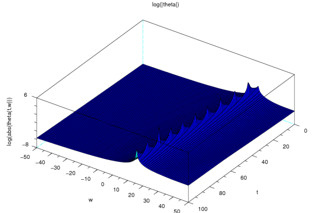
Fig. 8. Repartition of the peaks of \theta(t, w) . They all lie on the green line represented on Fig. 7. Normally, they should form a continuous crest, but due to discretization they show an uneven behavior.
