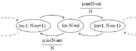
Fig. 4. Diagram of the Markovian transitions.
