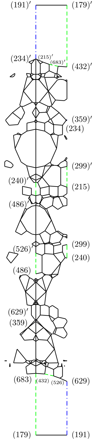
Figure 9: Fundamental domain in the case m = 191 . The coordinates of the vertices can be displayed by [39].
