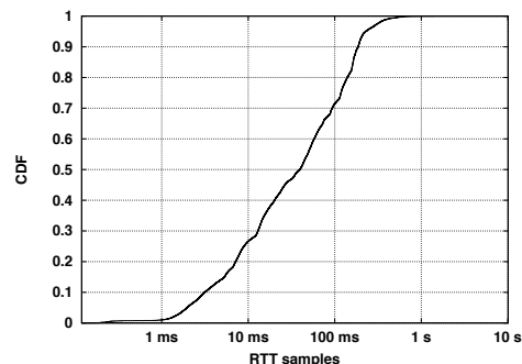
Figure 1: RTT distribution
